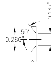
DETAIL A SCALE X3 VIEW SIDE VIEW
