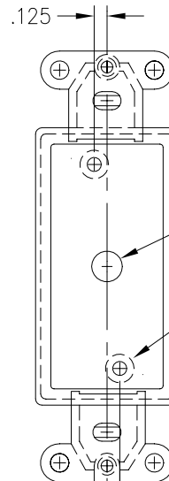
BACK VIEW
