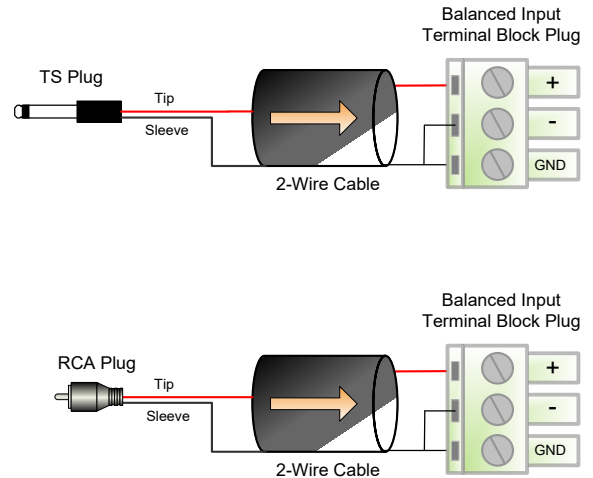
Figure 2 – Unbalanced Wiring Guide
