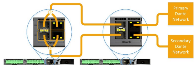
Figure 4 - “Redundant” mode with daisy chaining
