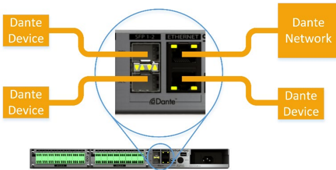
Figure 6 - "Standalone" connection in "Switched" mode
