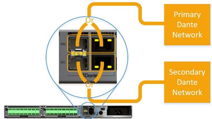
Figure 3 – “Redundant” mode, no daisy chain
